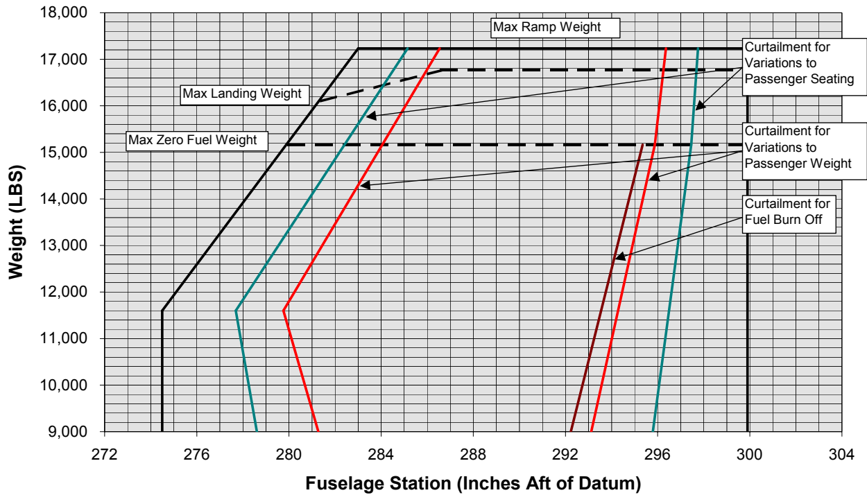
I FIGURE 3-5. OPERATIONAL LOADING ENVELOPE WITH A CURTAILMENT FOR VARIATIONS IN PASSENGER SEATING
